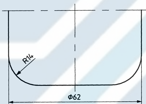
Figure A.3 — Profile of detachable blades
